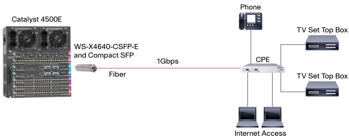
Figure 5. Compact SFP Deployment with Cisco Catalyst 4500
