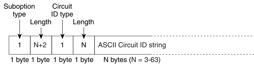
Figure 21-3 User-Configured Suboption Packet Formats
