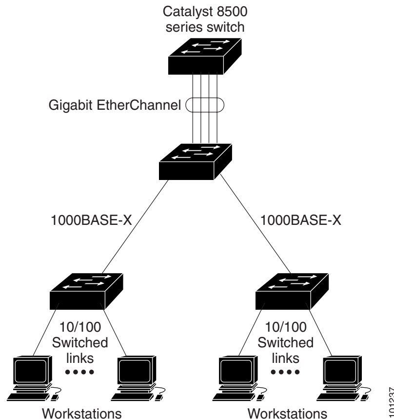
Figure 37-1 Typical EtherChannel Configuration
