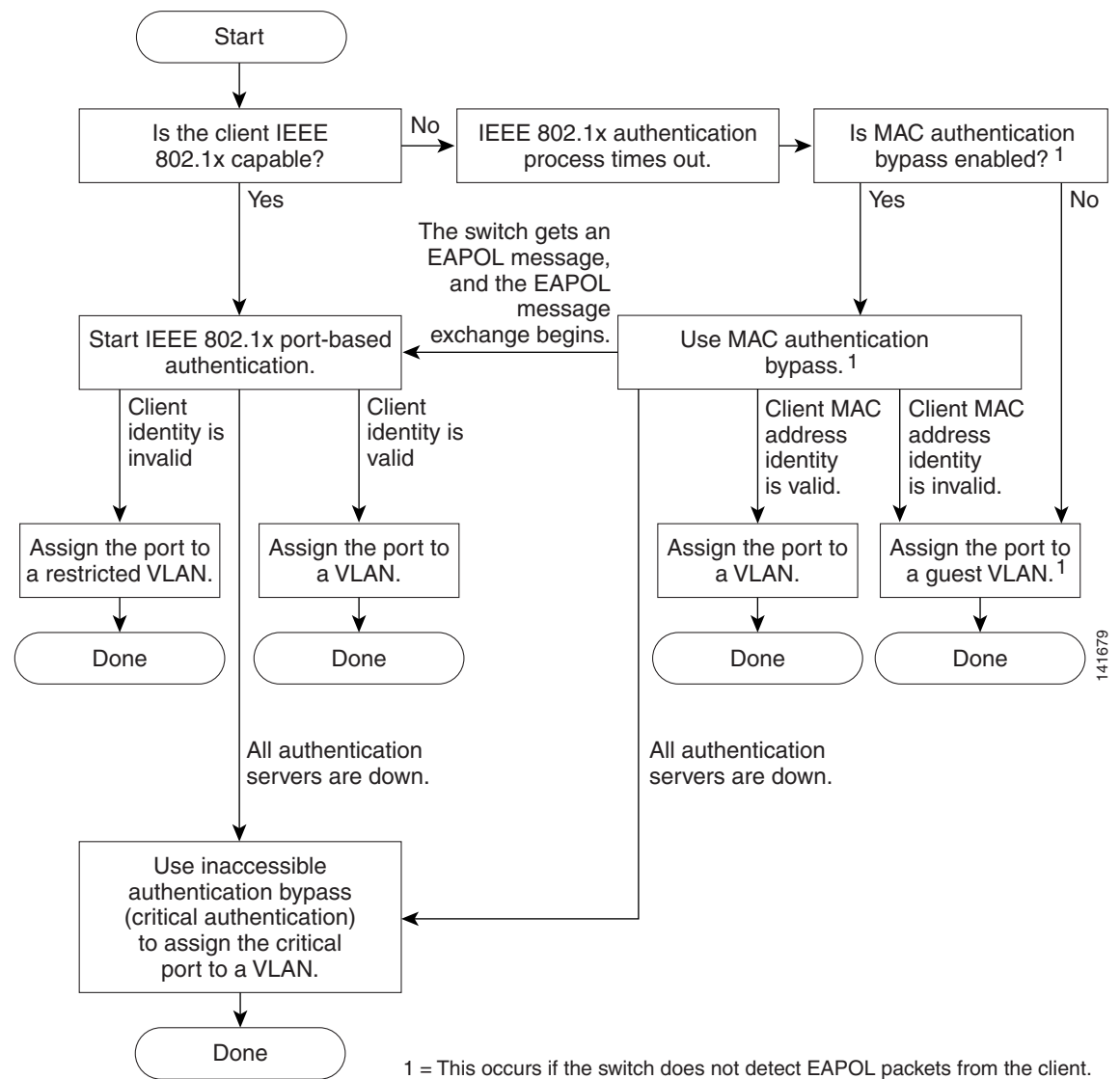
Figure 10-2 Authentication Flowchart
